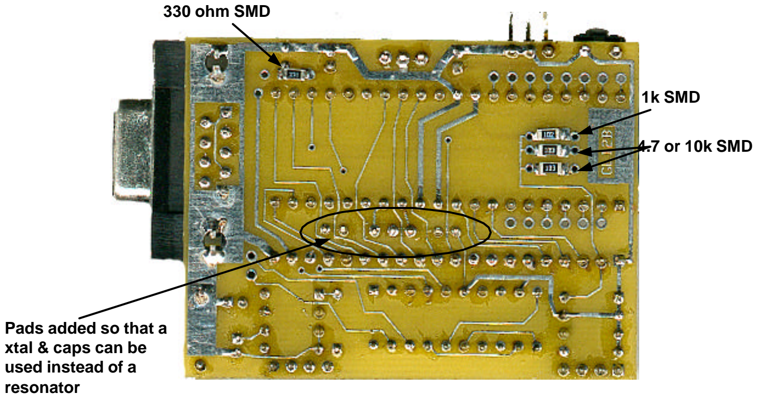
BOTTOM SIDE OF GLI2 Rev B pcb
