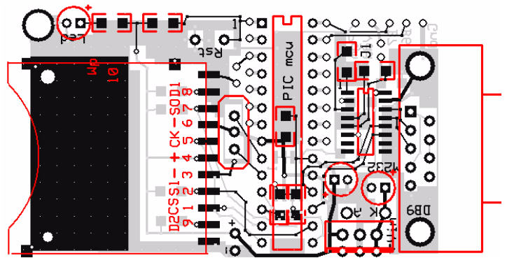
Printed circuit board layout
