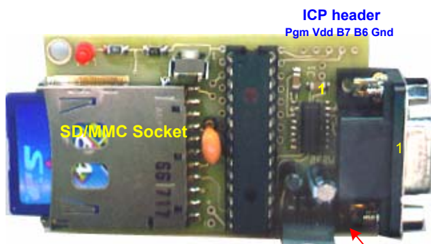
Assembled board (shown with a card)
