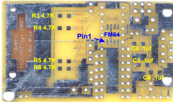
Bottom Side of pcb
