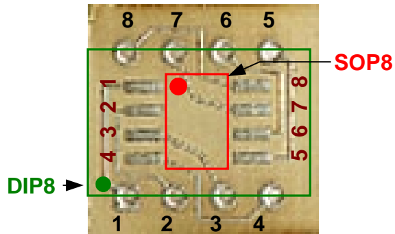
Pin to pin connections
