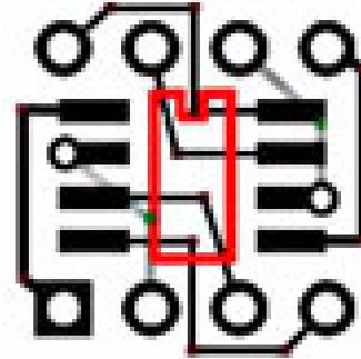
PCB Layout
