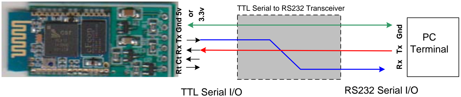
3,3v or 5v TTL to RS232 adapter
